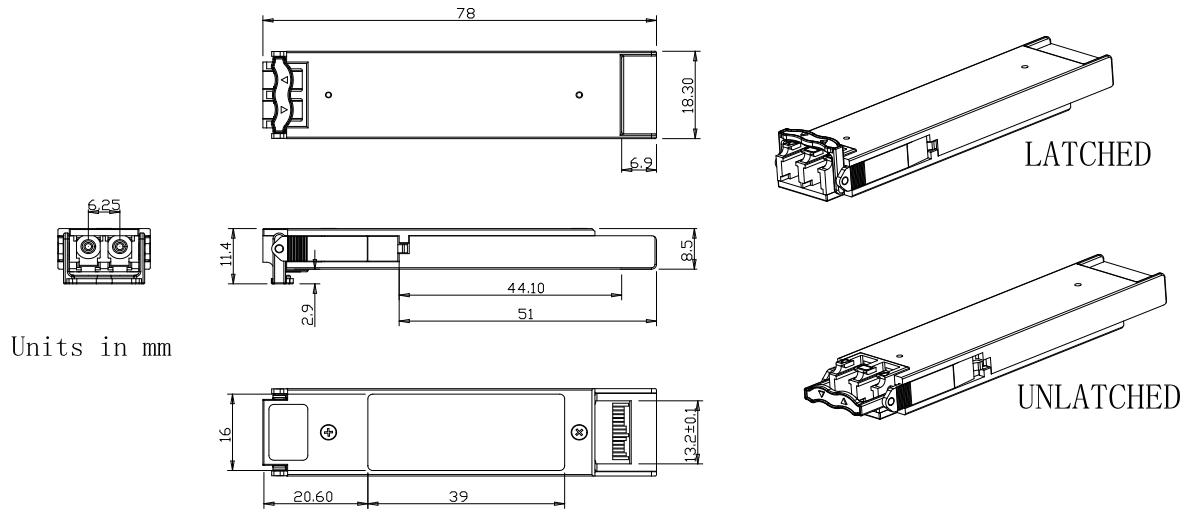
Transceiver (dimensions are in mm)
