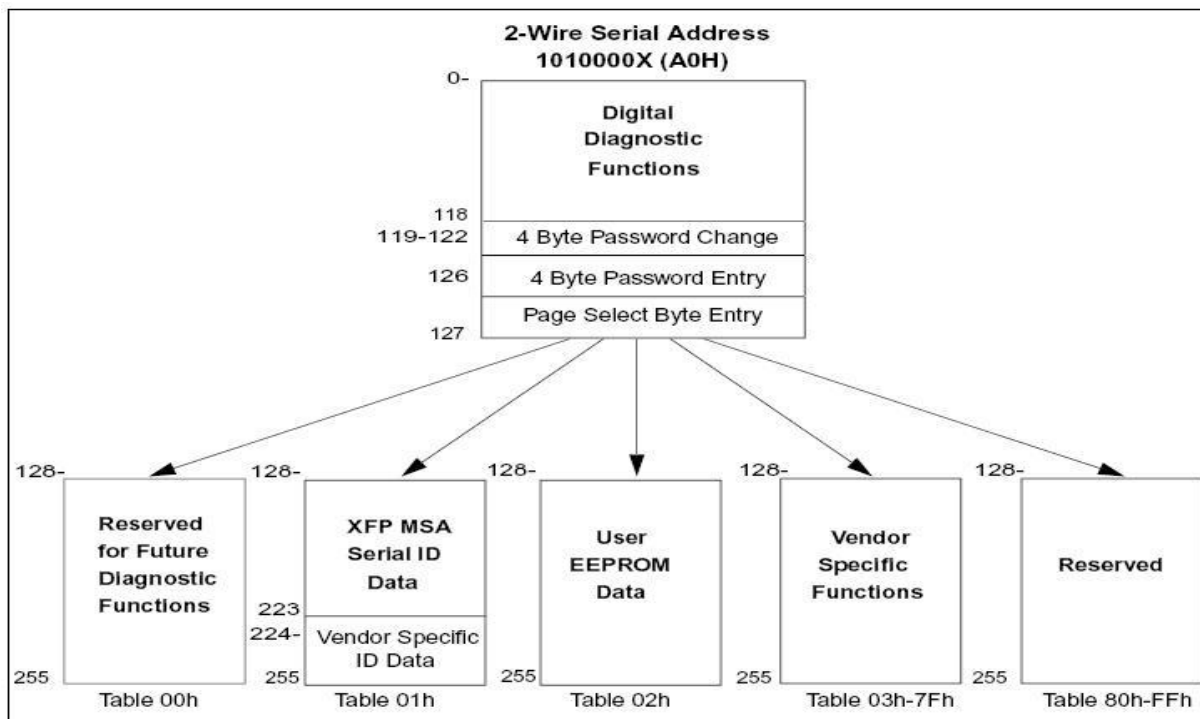
XFP two-wire serial digital diagnostic memory map
