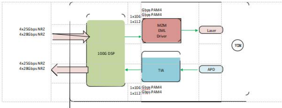
Figure 1. Block Diagram
