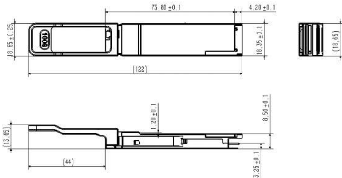
Figure 3. Mechanical Schematic
