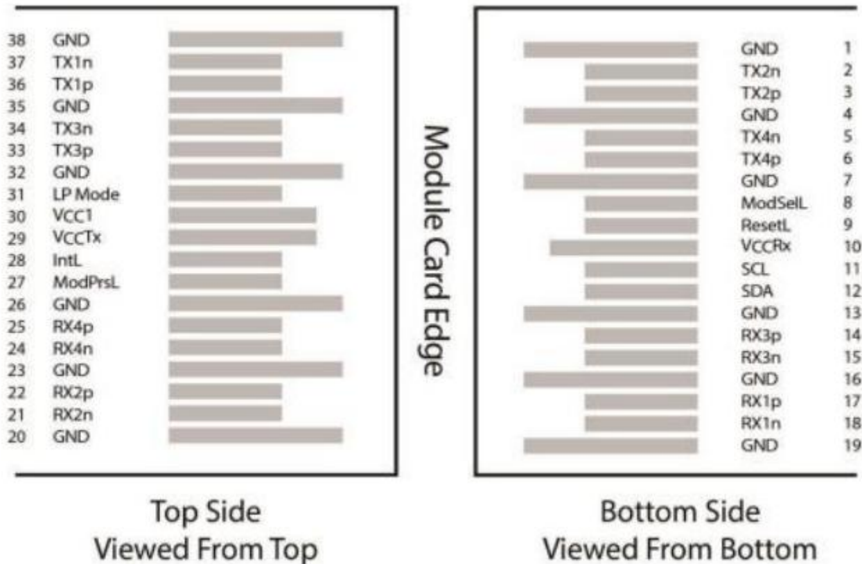
Figure 2. QSF28 Connector Pad layout
