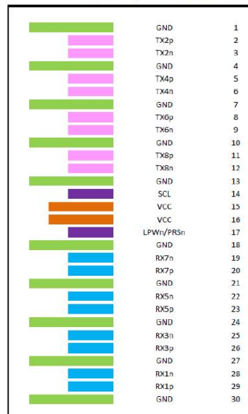
Bottom Side (viewed from bottom)
