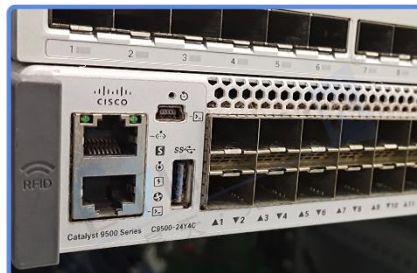
CISCO Catalyst 9500
