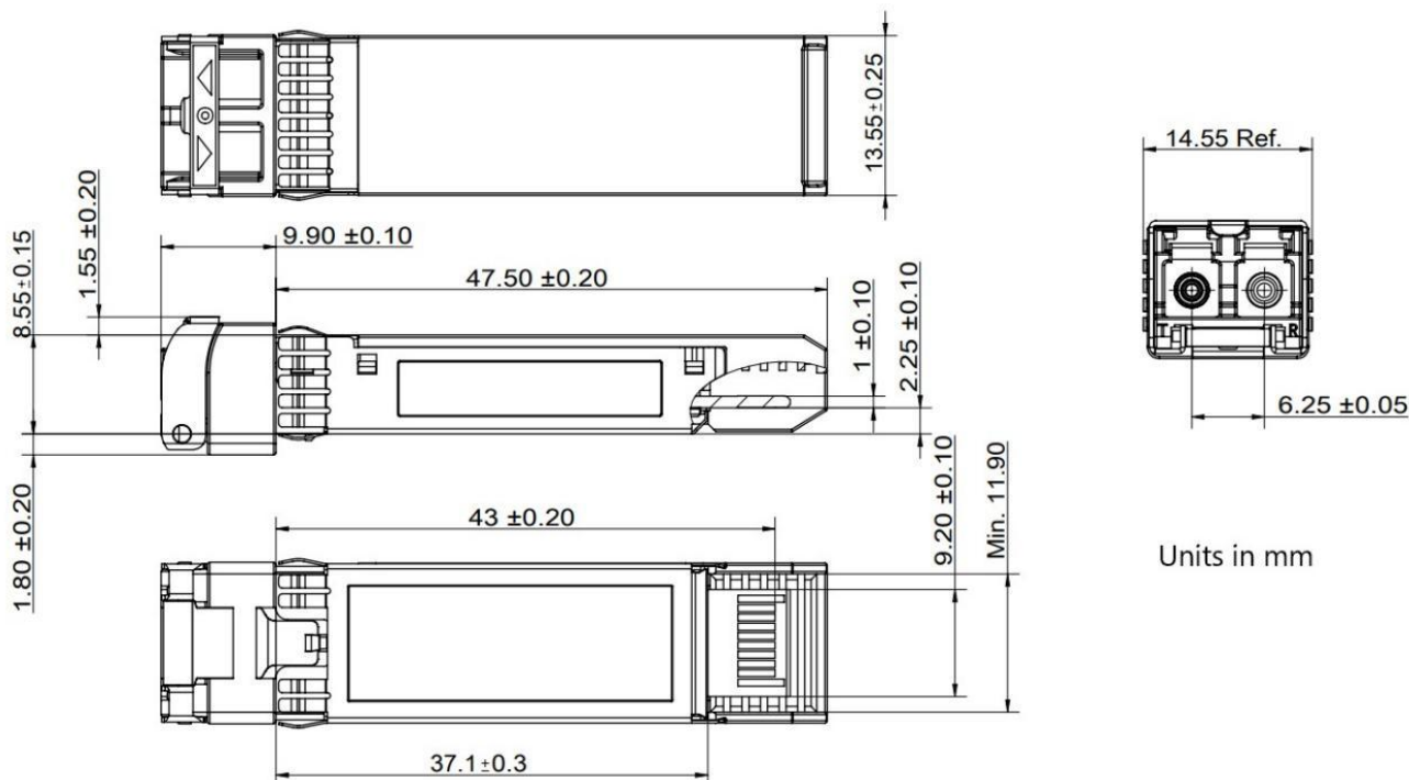
Figure2. Mechanical Outline
